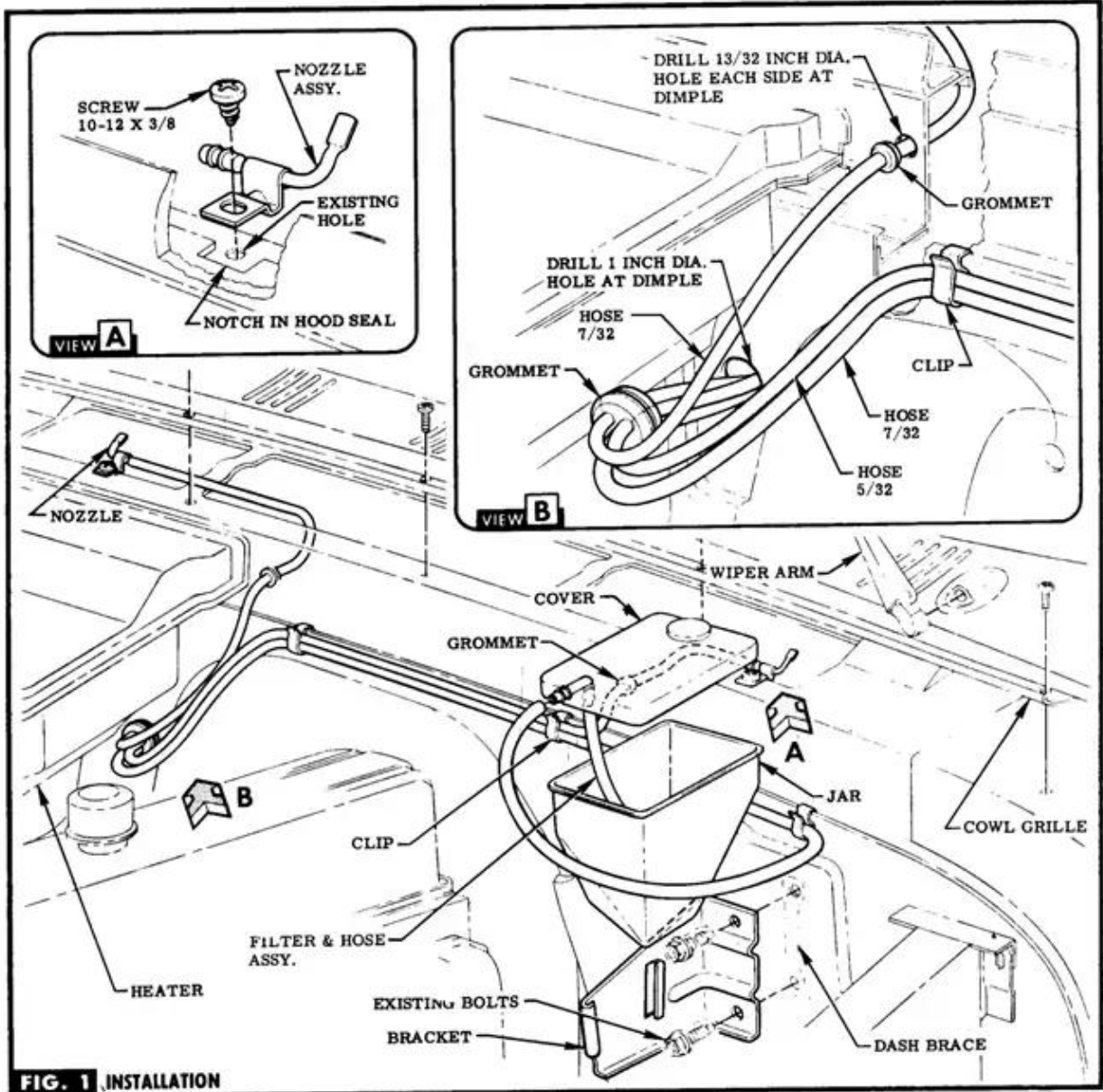
FIG. 1 INSTALLATION
