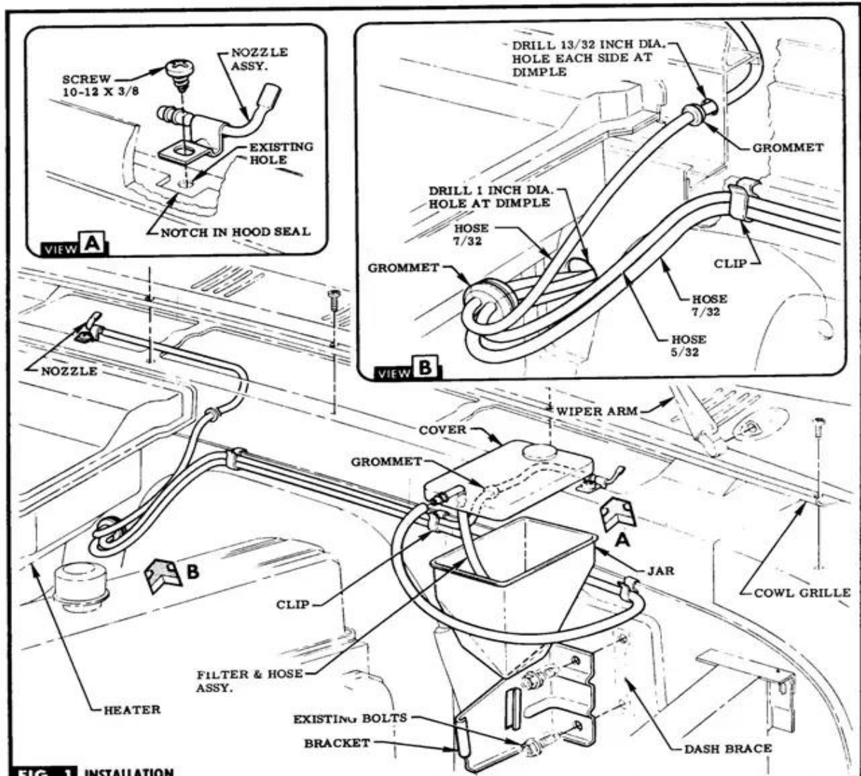
FIG. 1 INSTALLATION
